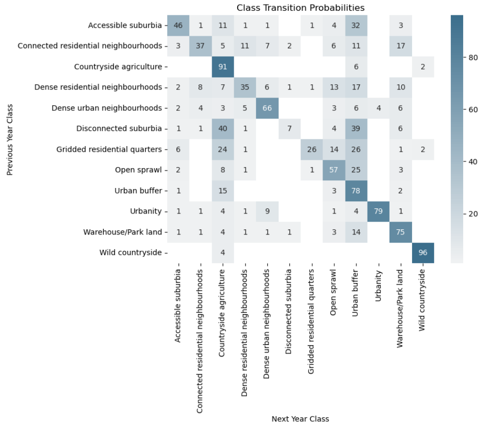
Figure 4.5: Class Transitions
