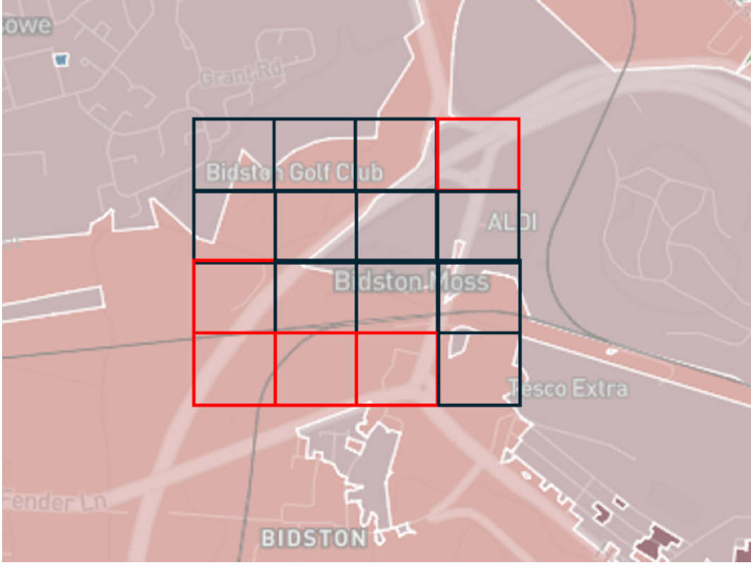
Figure 3.1: Sampling Strategy
