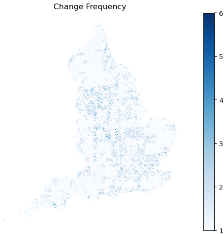
Figure 4.4: Frequency Map
