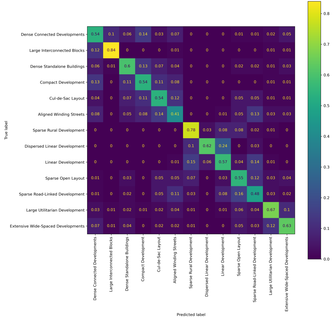
Figure 2.3: Confusion matrix for the Spatial model Level 4 predictions. Normalised by the True Label (row-wise)
