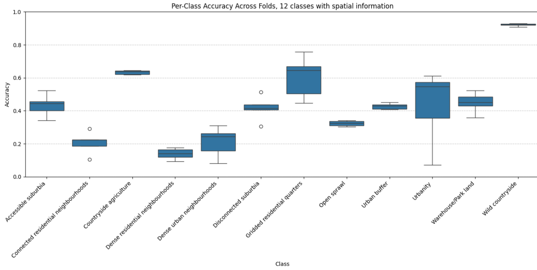
Figure 4.1: Per class accuracy, 12 classes with spatial context
