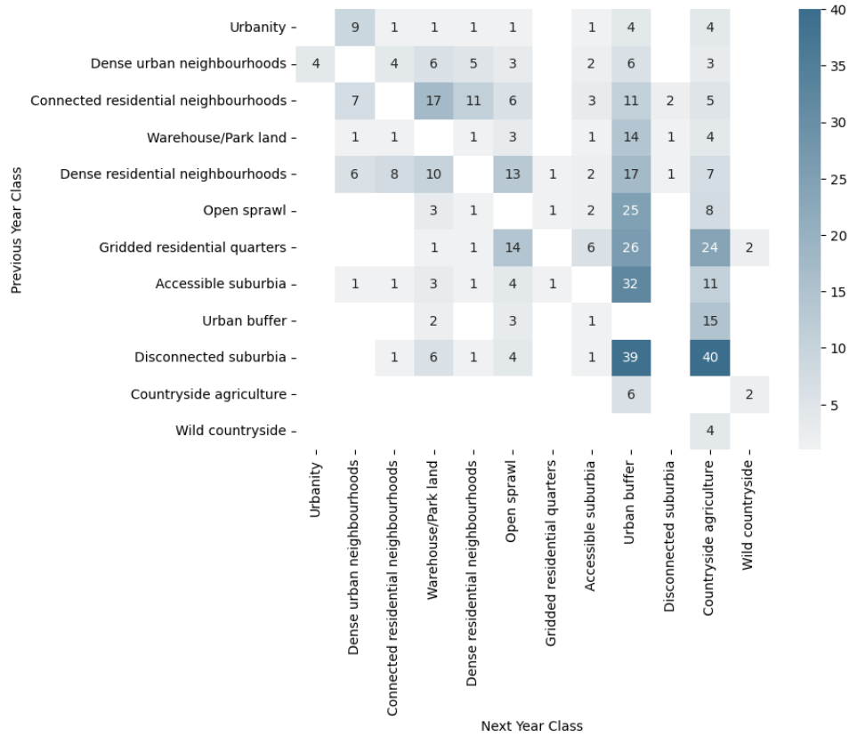
Figure 4.6: ‘Reasonable’ confusion matrix
