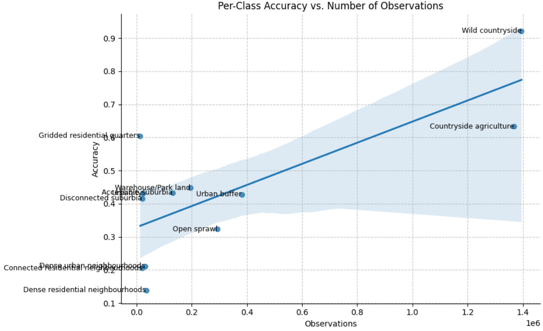
Figure 4.3: Number of observations vs accuracy
