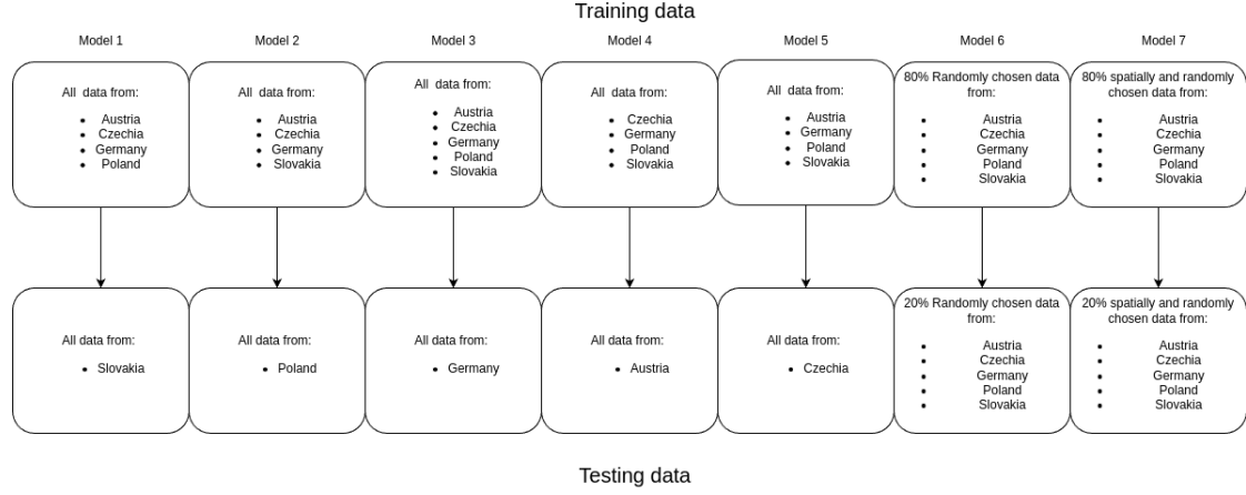
Figure 2.1: Train/test data splits for different models.
